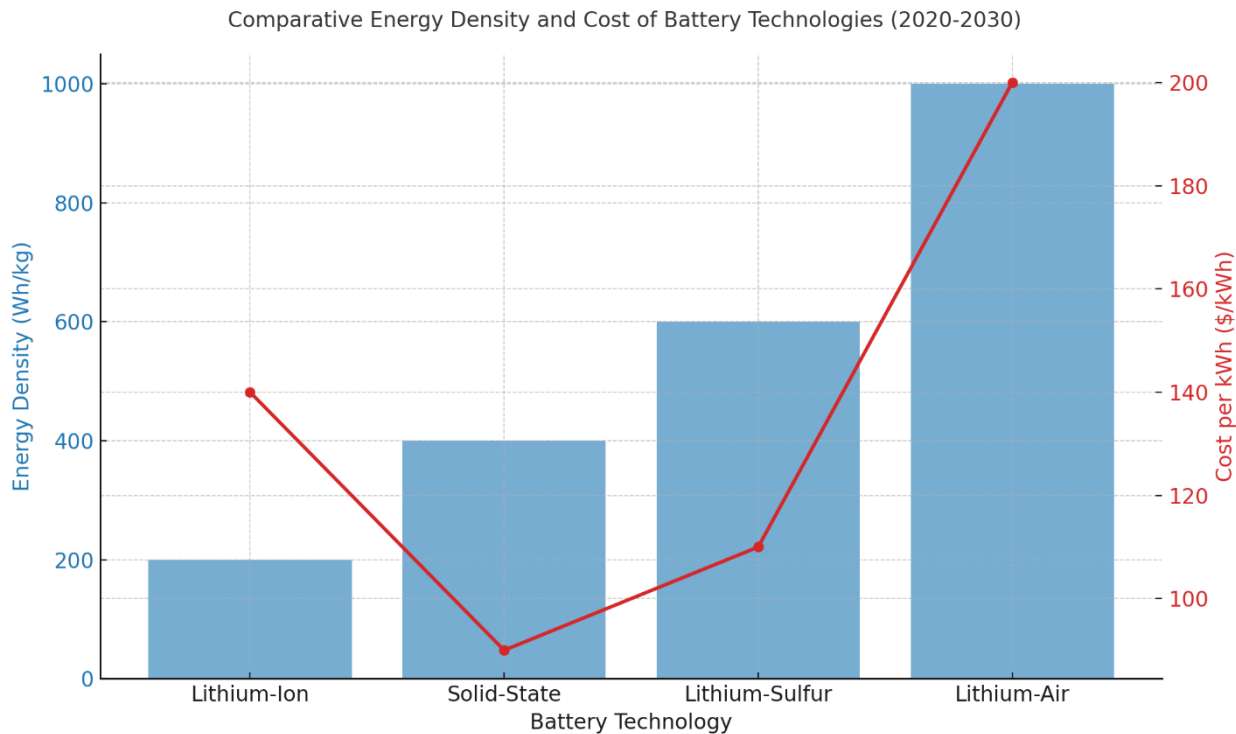
Figure 1 : Comparative Energy Density and Cost of Battery Technologies (2020-2030).
